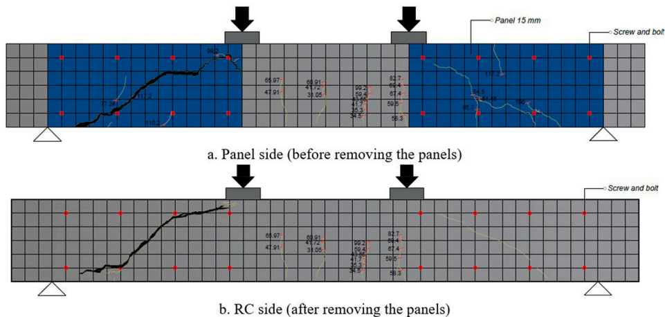
Fig. 16. Crack pattern of PM-W-200.
