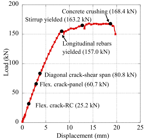
Fig. 23. Load-displacement of GM-W-200.
